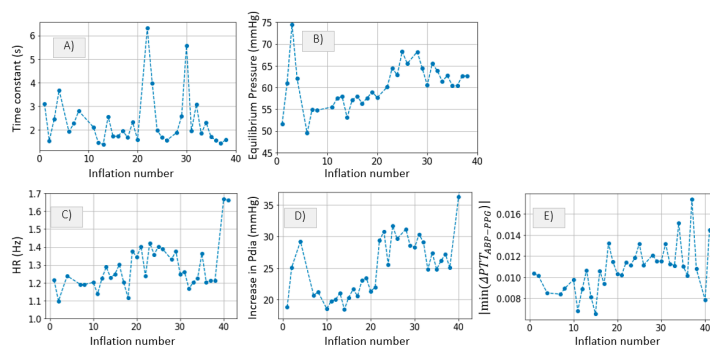
Figure 18. (A) Time constant \tau and (B) P_{Equilibrium} from Patient 1 data. (C) HR, (D) increase in P_{dia} and (E) maximum drop in \Delta PTT_{ABP-PPG} are plotted for qualitative comparison.
