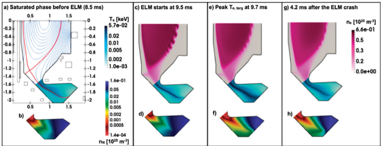
Figure 49. The simulation of an ELM crash in MAST Upgrade is shown. The simulations are performed using the neutrals model available in JOREK. The originally detached state with low target temperatures (left plot) is re-attaching during the ELM crash in the Super-X divertor (right plots). Reproduced from [77]. CC BY 3.0.
