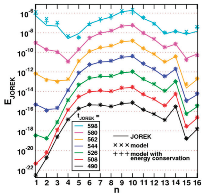
Figure 36. For various time points during a JOREK simulation (times in JOREK units), the toroidal mode spectrum is shown. The linearly most unstable mode numbers around n = 10 give rise to a broad mode spectrum in the non-linear phase at the ELM onset driven by non-linear mode coupling. In particular the linearly stable n = 1 mode is driven to amplitudes comparable to the linearly dominant n = 10 mode. Reprinted from [201], with the permission of AIP Publishing.
