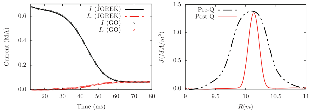
Figure 24. (Left) Time evolution of the total plasma current I and the RE current I_r during the current quench phase. (Right) Midplane current density profiles before and after the current quench obtained from JOREK, showing a relatively peaked RE current profile. Reprinted figure with permission from [111], Copyright 2019 by the American Physical Society.
