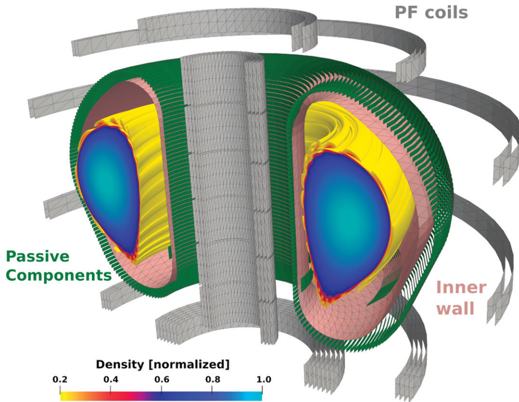
Figure 44. The perturbed density during an ELM crash induced by a vertical magnetic kick is shown. All relevant conducting structures were included in the JOEKE–STARWALL simulation. The figure was generated based on the simulation data published in reference [171].
