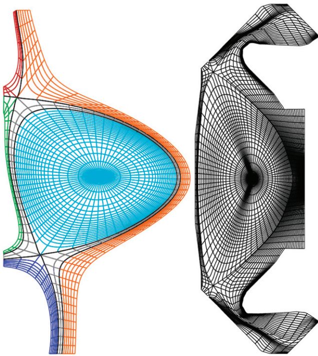
Figure 6. JOEUK example grids shown at reduced resolution for clarity. (Left) Flux-surface aligned grid [123] for a TCV equilibrium with two X-points (the lower X-point is active). The part in the closed flux region is shown in light blue, the two separatrices in black, the grid between the separatrices in grey, the lower private flux region in dark blue, the upper private flux region in red, the outer open flux region in orange, and the inner open flux region in green. (Right) Flux surface aligned X-point grid extended to the true first wall (using the methods described in reference [124]) for an MAST Upgrade case with Super-X divertor.
