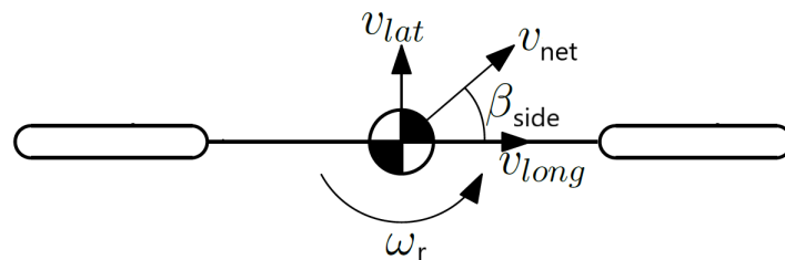
Figure 3.4: 3 DOF bicycle model
