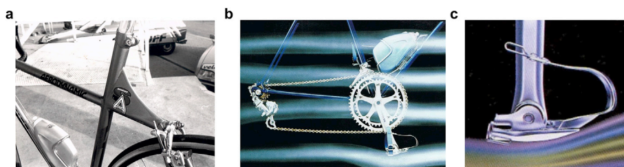
Fig. 34. (a) Aerodynamic appendices behind the seat tube in the aerodynamic Schauf bicycle (reproduced with permission from Schauf); (b) Shimano first aerodynamically optimized group-set (source: Shimano catalogue 1980); (c) Detail of the aerodynamically optimized pedal by Shimano (source: Shimano catalogue 1981).
