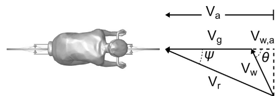
Fig. 6. Cyclist velocity definitions: V_g is the ground or cyclist velocity, V_w is the wind velocity, V_{w,a} is the wind velocity component in the riding direction, V_r is the relative velocity, V_a is the relative velocity component in the riding direction, \psi is the yaw angle, \theta is the wind angle.
