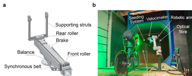
Fig. 12. (a) Force balance used for cycling aerodynamics testing that enables the rotation of the rear wheel and of the front wheel by a belt (source: Gibertini and Grassi, 2008; reproduced with permission from Springer Nature); (b) Particle image velocimetry (PIV) technique used by Jux et al. (2018) in the open jet wind tunnel at Delft University of Technology in the Netherlands (source: Jux et al., 2018; CC BY 4.0).
