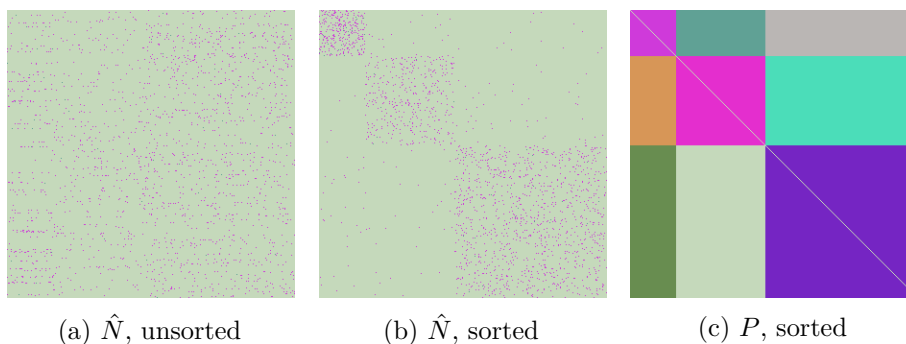
Fig 4: A sample path of length T = n^{1.025} \ln n \approx 1973 was generated, from which \hat{N} is calculated. If we sort the states according to the clusters they belong to, we can see that states within the same cluster share similar dynamics.
