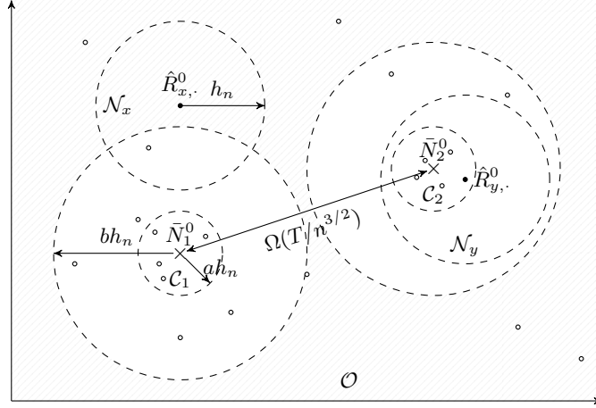
Fig 9: Schematic depictions of cores \mathcal{C}_1, \mathcal{C}_2 for K = 2 , the set of outliers \mathcal{O} (shaded area), and neighborhoods \mathcal{N}_x, \mathcal{N}_y for some x \in \mathcal{O} and y \in \mathcal{C}_2 .
