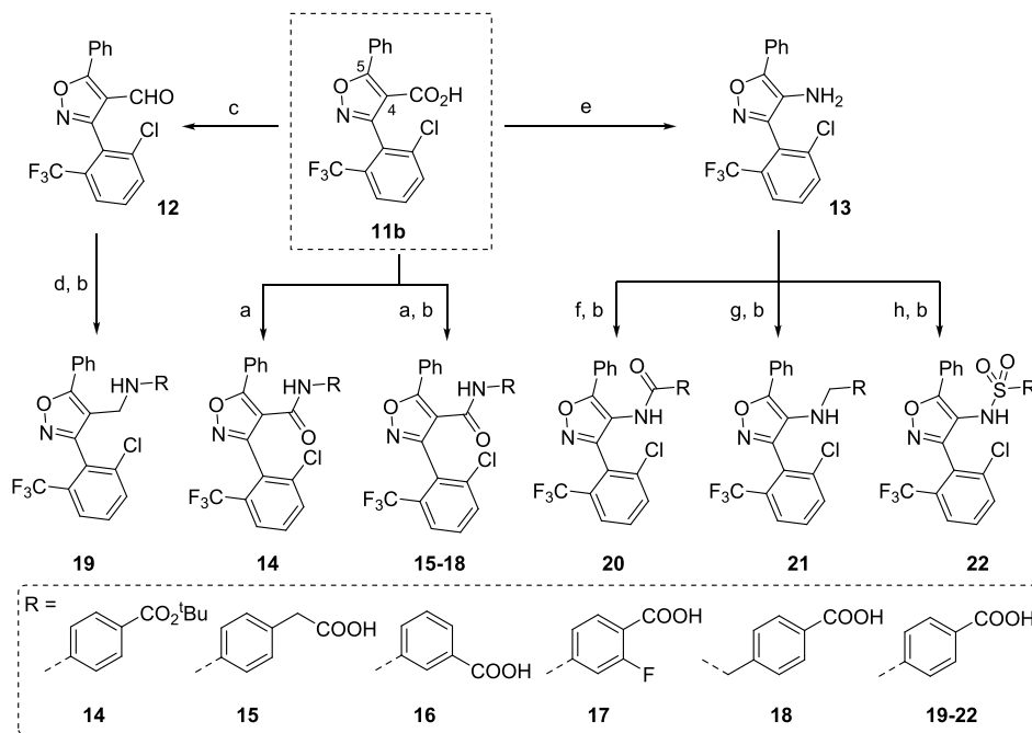
Scheme 2. Synthesis of C-4 Isoxazole Derivatives a
