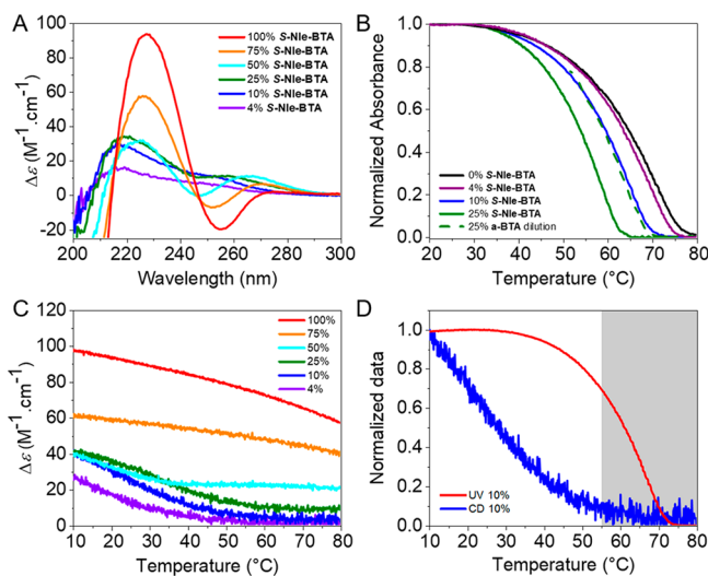
Figure 1. (A) CD spectra of the mixture a -BTA and S -Nle-BTA at c_{\text{tot}} = 50 \mu\text{M} in MCH at 20 ^\circ\text{C} . (B–C) Temperature-dependent UV (B) and CD (C) spectra of solutions containing different ratios of S -Nle-BTA/ a -BTA probed at \lambda_{\text{max}} with c_{\text{tot}} = 50 \mu\text{M} in MCH (cooling rate = 2 \text{K}\cdot\text{min}^{-1} ). (D) Normalized CD and UV cooling curves probed at \lambda_{\text{max}} with c_{\text{tot}} = 50 \mu\text{M} in MCH at the ratio of S -Nle-BTA/ a -BTA 1/9.
