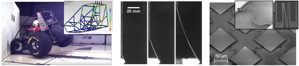
(a) Car safety frame crash test 1 and simulation (Reproduced from [53]) (b) Projectile wire test (Reproduced from [38]). (c) Deforming stretchable electronic interconnects; horseshoe-shaped and rectangular design
