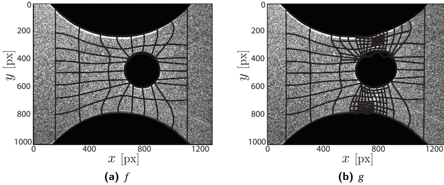
Figure 2.14: Images of the sample before and after deformation, as used in the correlation process. The mesh before and after refinement is also shown.
