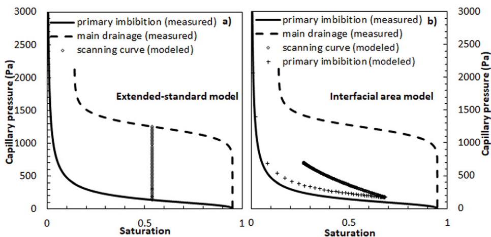
Fig. 7. Pressure-saturation curves corresponding to (a) the extended-standard (ESD) model and (b) the interfacial area (IFA) model.
