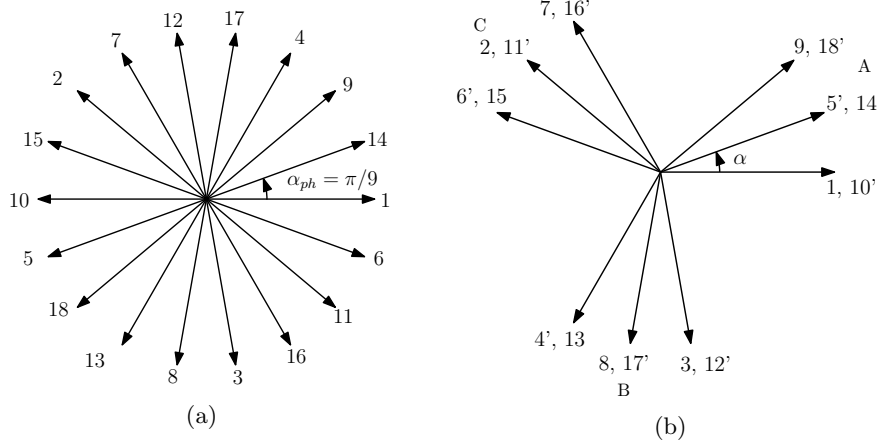
Figure 4.14: The 18/20 VFRM: (a) the original phasor diagram of the flux linkage assuming all the coils are in the same orientation, and (b) the winding configurations ( p_s/m = 3 ).
