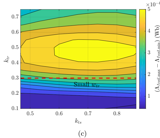
Figure 4.19: The values of coil flux linkage ( \Lambda_{fcoil,max} - \Lambda_{fcoil,min} ) by varying stator and rotor teeth widths in (a) 12/10 VFRM, (b) 12/22 VFRM, and (c) 12/2 VFRM ( k_{ts} and k_{tr} are the ratios of the stator/rotor tooth width to stator/rotor slot pitch).
