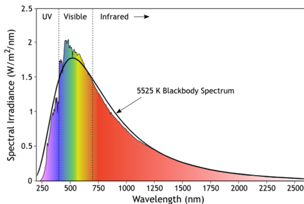
Figure 15. Spectral irradiance of sunlight.
