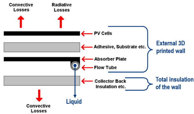
Figure 11. Diagram model of the Spong3D system in Trnsys, which is applied as a vertical wall system. The existing PV layer of the Trnsys Type 560 was given the same thermophysical properties as the Spong3D material.
