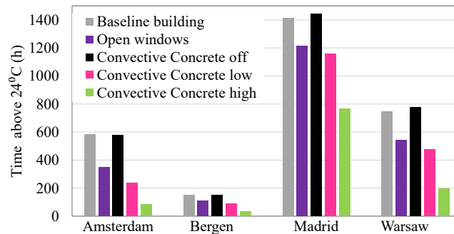
Figure 5. Hours above 24 °C for four locations.
