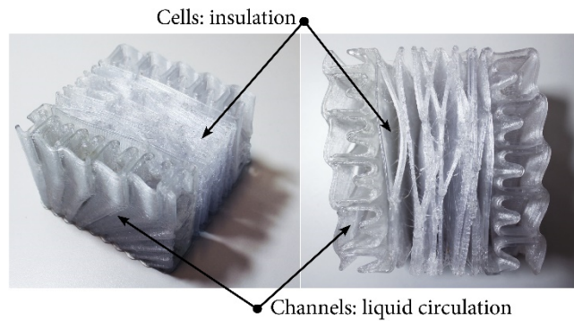
Figure 8. Sample of the structure with its channels and cells.
