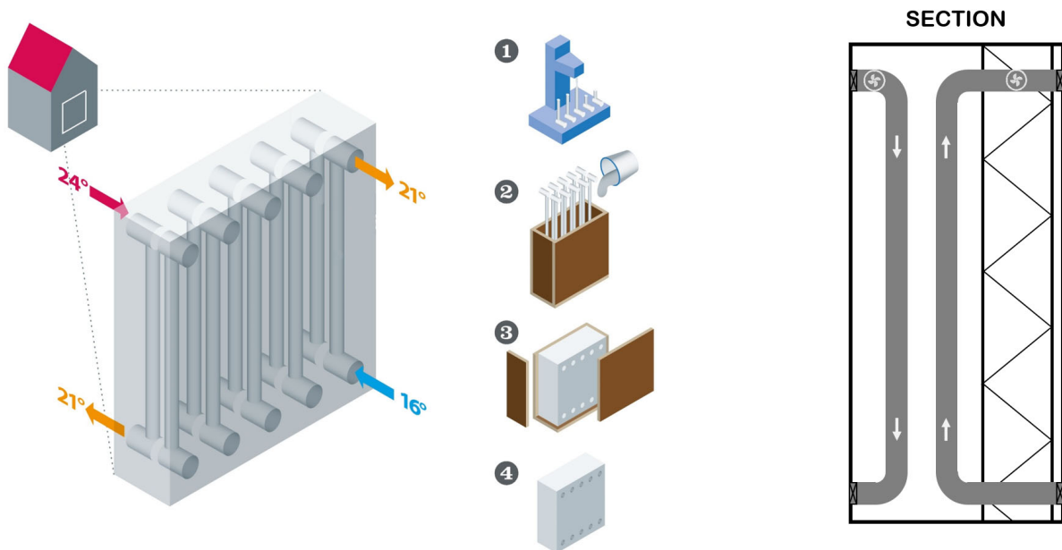
Figure 1. Convective Concrete concept.
