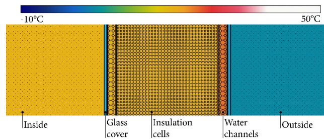
Figure 10. Model of the Spong3D system with glass cover in Energy2D (section).
