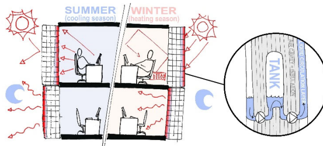
Figure 9. Schematic illustration of the operation of the system.
