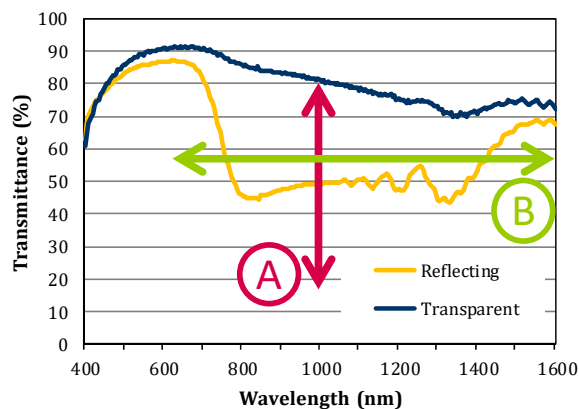
Figure 14. Spectral transmittance of the switchable NIR reflecting layer.
