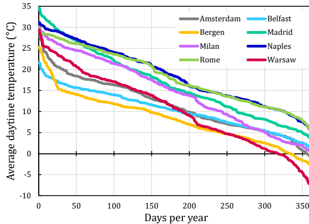
Figure 6. Temperature duration curves of average daytime (08h00 – 18h00) outside temperature.
