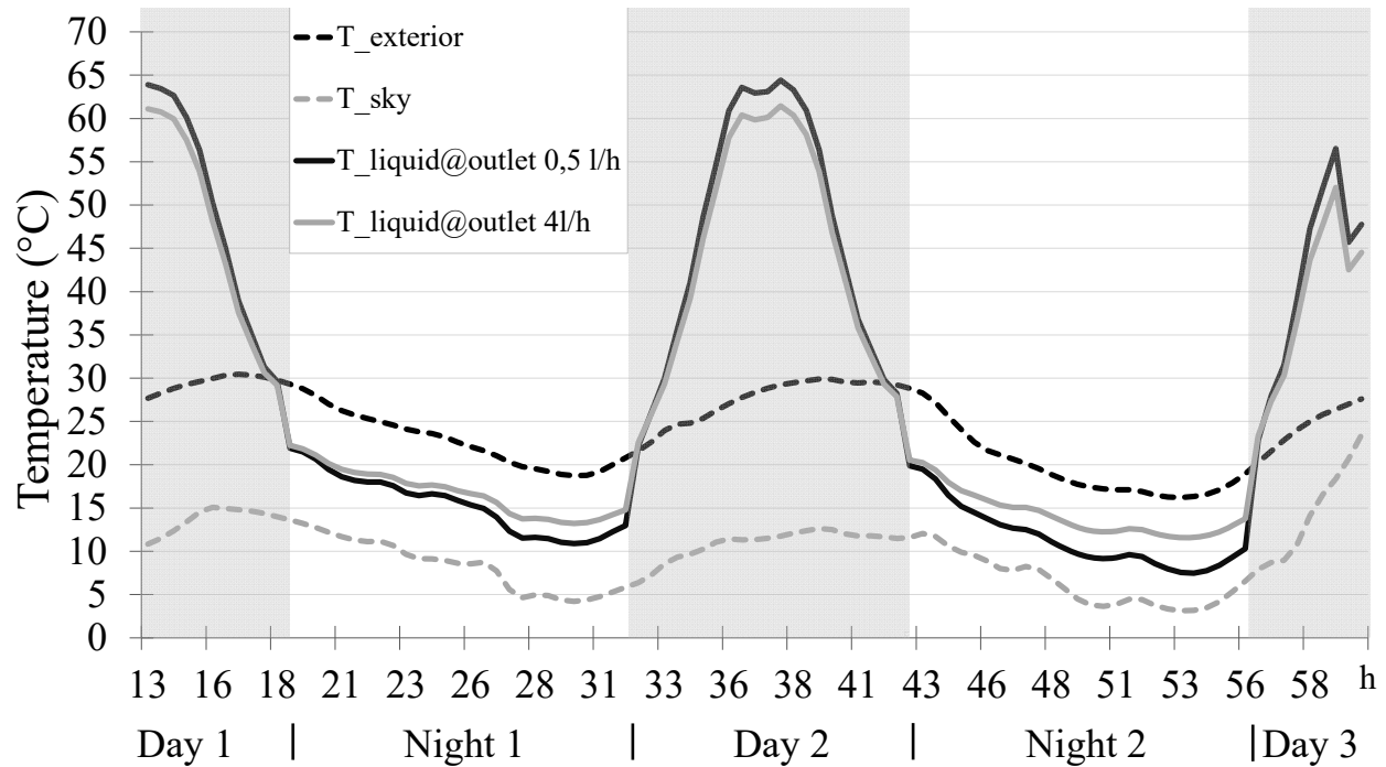
Figure 12. Trnsys results showing the temperature of the liquid during two summer nights for two mass flow rates.
