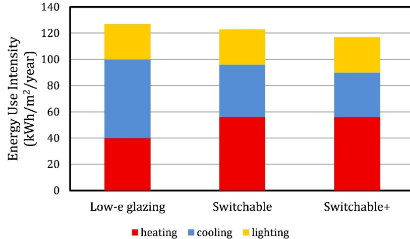
Figure 17. Comparison of the energy-saving potential of (i) a reference glazing system (low-e), (ii) the current generation NIR-reflecting switchable glazing system, and (iii) the NIR-reflecting switchable window with enhanced spectral properties.
