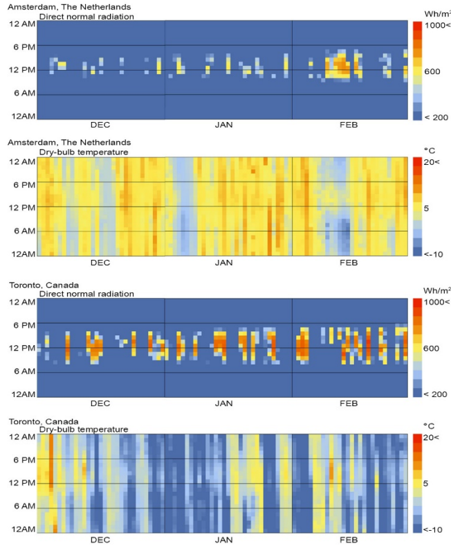
Figure 13. Radiation and temperature flood chart for Amsterdam (top) and Toronto (bottom).
