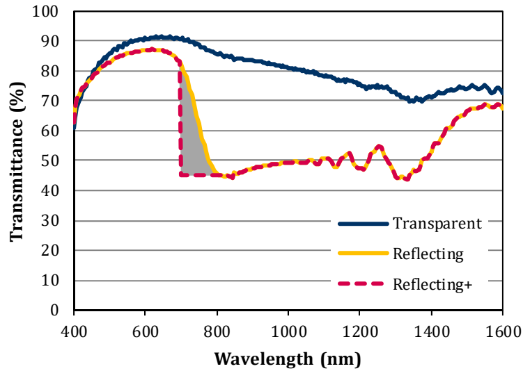
Figure 16. The reflecting+ film has a sharp cut-off wavelength at 700 nm.
