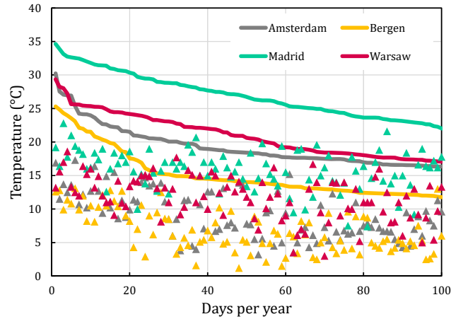
Figure 7. Temperature duration curves with daily temperature amplitude on the corresponding day.
