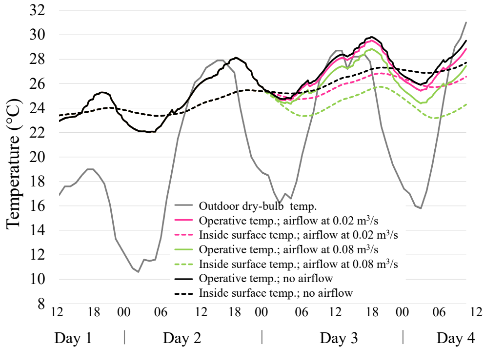
Figure 4. Effect of the Convective Concrete with an air flow rate of 0.02 and 0.08 \text{ m}^3/\text{s} compared to the system off.
