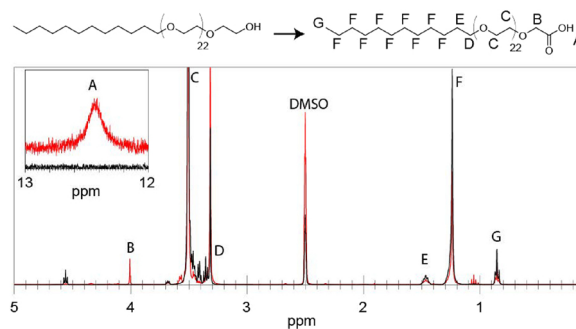
Fig. B.10. 1 H NMR of unmodified Brij 35 (top left, black) and ModBrij 35 (top right, red) (400 MHz, DMSO-d 6 ): δ 12.60 (broad s, 1H), 4.01 (s, 2H), 3.51 (m, 88H), 3.32 (m, 2H), 1.47 (p, J = 8 Hz, 2H), 1.24 (m, 18H), 0.85 (t, J = 8 Hz, 3H). The conversion is computed from the ratio of the integrals of protons B and G, which gives a conversion of 95%.
