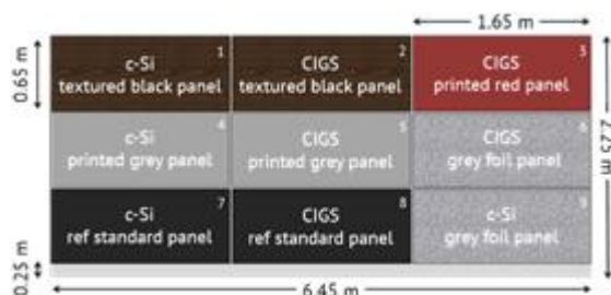
Figure 1: Schematic representation of the colored PV façade demonstrator.
