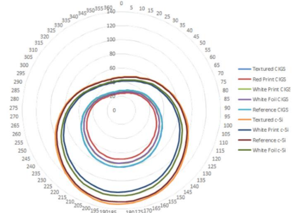
Figure 12: Simulation results for PV façades located in Amsterdam, of various PV technologies and orientations with various colors and textures. The annual yield is in kWh/m 2
