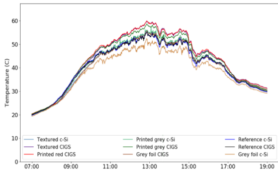
Figure 9: Module temperatures of the 9 PV panels composing the prototype PV facade demonstrator, on July 16, 2018.
