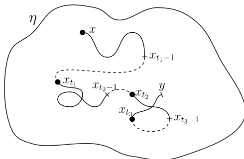
FIG. 4. An example of a segmented path with 4 segments. Solid lines represent the segments, consisting of a path of half-edges in \eta , dashed lines indicate the succession of the segments. The latter do not necessarily correspond to a pair in \eta , and will later correspond to rewired edges in the graph dynamics.
