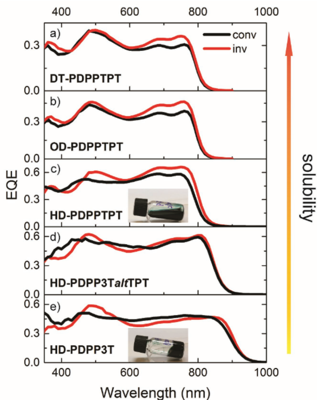
Figure 3. EQE of a) DT-PDPPPTPT:[70]PCBM, b) OD-PDPPPTPT:[70]PCBM, c) HD-PDPPPTPT:[70]PCBM, d) HD-PDPP3TaltTPT:[70]PCBM, and e) HD-PDPP3T:[70]PCBM with conventional (conv.) and inverted (inv.) polarities. For each layer the polymer:fullerene weight ratio was 1:2. Chloroform was used as the main solvent for processing in all cases. From bottom to top, the solubility of polymer is increasing. The weight average molecular weight ( M_w ) of HD-PDPP3T is 400 \text{ kg mol}^{-1} . The image in the bottom panel shows gel formation within 2 h due to the limited solubility, while the more soluble polymer (middle panel) remains well dissolved.
