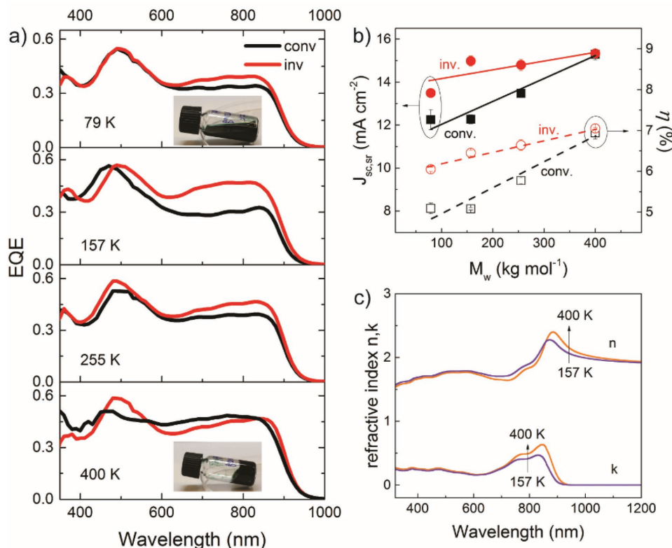
Figure 5. a) EQE spectra of HD-PDPPP3T :[70]PCBM blend (1:2 w/w) films with various M_w . The bottom inset image shows gel formation in 2 h due to the limited solubility, while low- M_w polymer (top inset) remains well dissolved in solution. b) The dependence of J_{sc,sr} and PCE ( \eta ) on M_w . The solid and dashed lines are guides to the eye. c) Refractive index ( n,k ) data of HD-PDPPP3T :[70]PCBM blend films.
