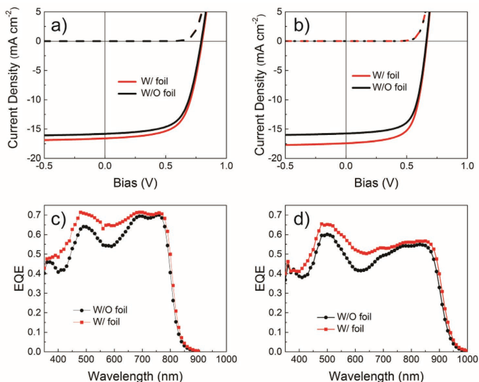
Figure 10. J - V characteristics and spectrally resolved EQEs of a,c) HD-PDPPTPT:[70]PCBM and b,d) HD-PDPP3T:[70]PCBM without (W/O) and with (W/) retroreflective foils.
