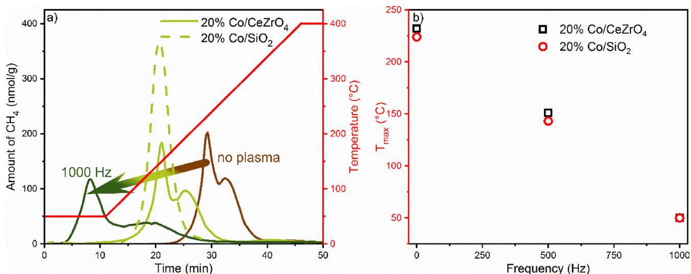
Fig. 12. CO hydrogenation in the presence of 20% Co/CeZrO 4 and 20% Co/SiO 2 catalysts by the TPPSR method: a) TPPSR profiles at different frequencies: 0, 500 and 1000 Hz; b) maximum temperatures of CH 4 formation. Pulse duration 90 μs.
