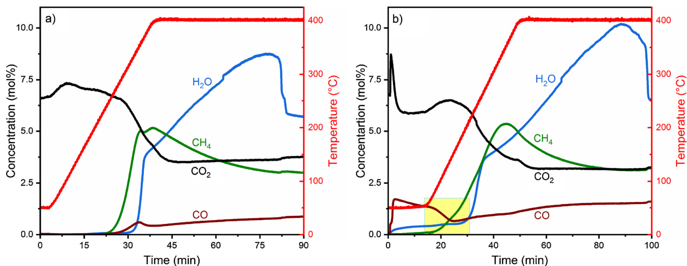
Fig. 6. CO 2 hydrogenation in the presence of 5% Co/CeZrO 4 catalyst by TPPR method: a) without plasma; b) in plasma, pulse duration 90 μs, frequency 1 kHz. CO 2 /H 2 /Ar = 1/4/10, total flow 75 ml/min, heating ramp 10 °C/min.
