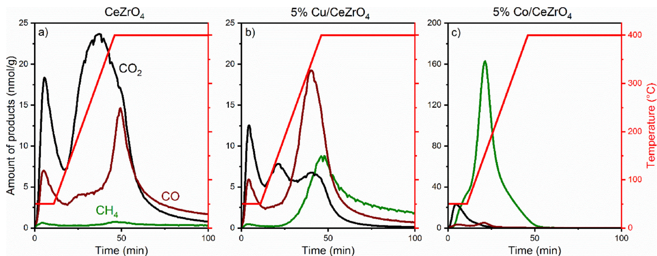
Fig. 8. TPPSR of \text{CO}_2 adsorbed on different \text{CeZrO}_4 -based samples in a \text{H}_2 flow: \text{CeZrO}_4 , 5% \text{Cu/CeZrO}_4 and 5% \text{Co/CeZrO}_4 at an energy density of 740 kJ/l.
