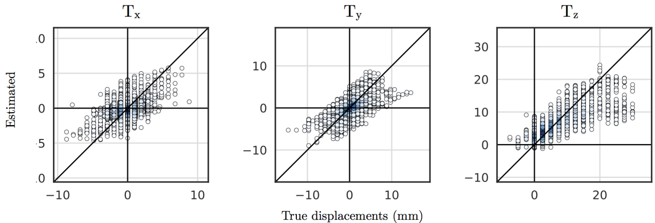
Figure 3. Correlation plots for each of the vector field components. Every point corresponds to a landmark in the ten test images. Darker colors indicate a higher density of points.
