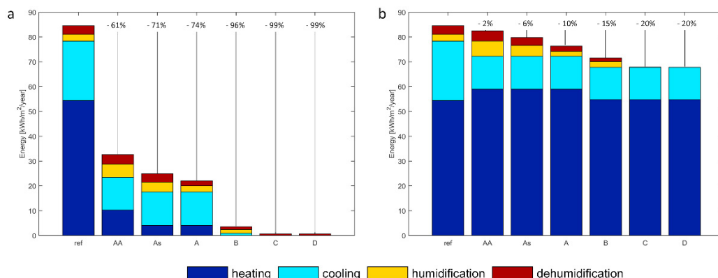
Fig. 2. (a) Specifications of energy demand and energy savings per ASHRAE climate class; (b) Conditioned according to T_{sp} = ATG during opening hours and ASHRAE's museum indoor climate classes during closing hours; for RH_{sp} ASHRAE's climate classes are used.
