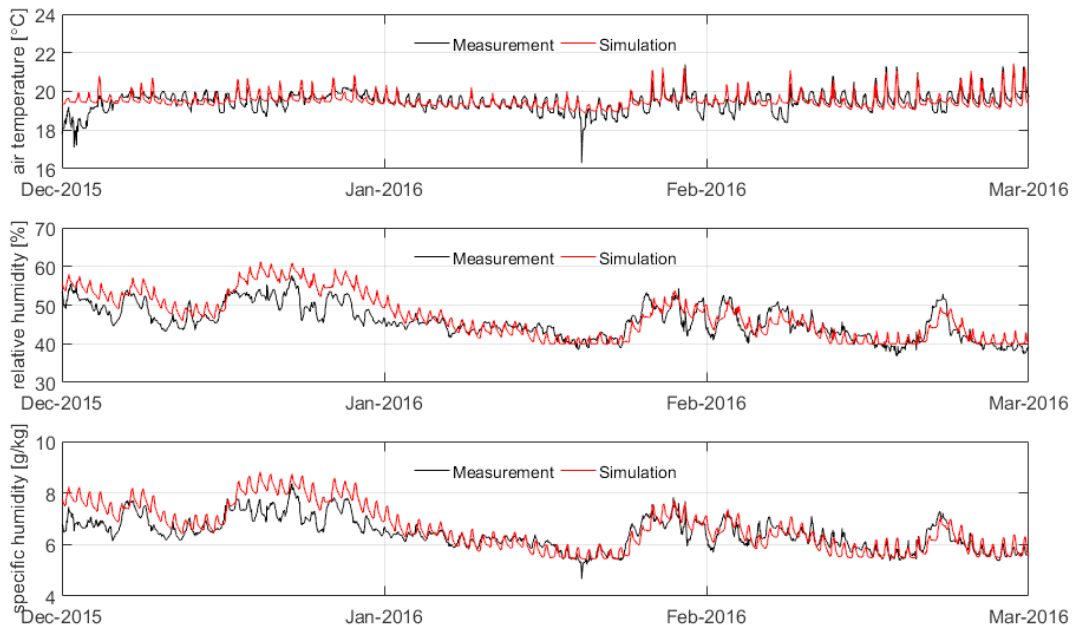
Fig. 1. Calibration results for temperature, relative humidity and absolute humidity.
