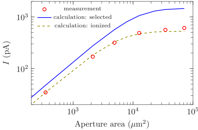
FIG. 9. Experimental data (markers) of the beam current plotted against the area of the aperture used to select the atomic beam. The data is taken at a Knudsen source temperature of 433 K, with I_i = 6 \times 10^9 \text{ W/m}^2 and s = 6000 . The lines show simulation data under the same conditions as the measurement. The solid line shows the current equivalent of the atomic flux that is transmitted through the selection aperture. The dashed line shows the current that is actually created. A fit is performed to find the current equivalent of the (unselected) incoming flux that matches the calculation data best with the experimental data, which resulted in 1.4 nA.
