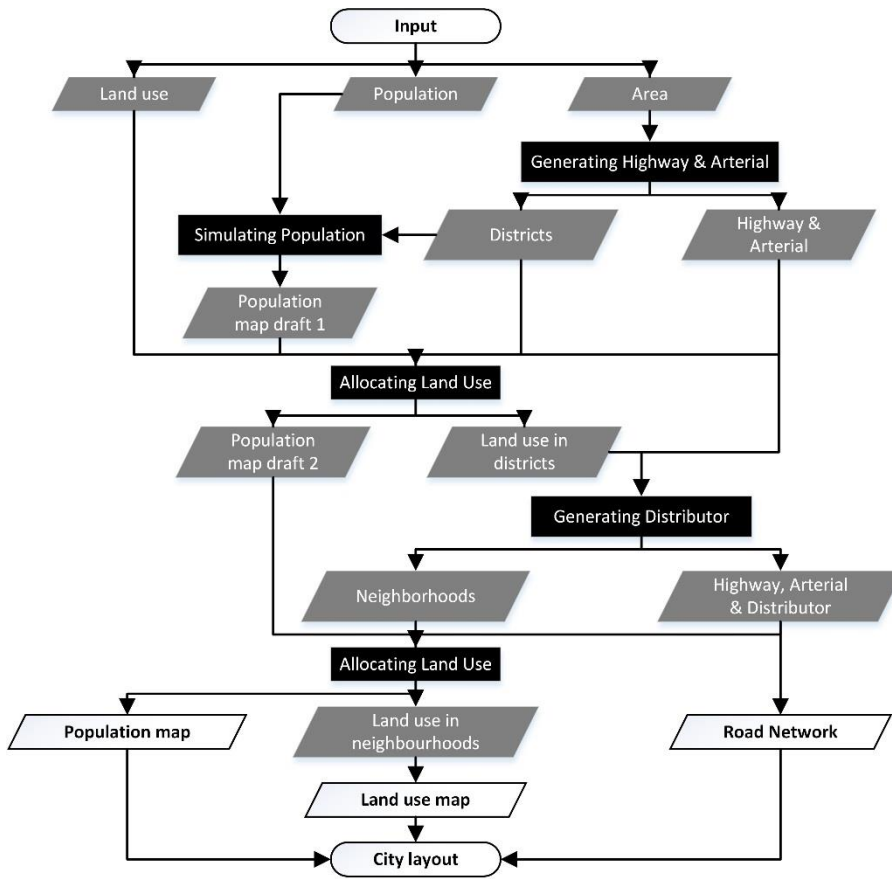
Fig. 1. The framework of the city simulation model.
