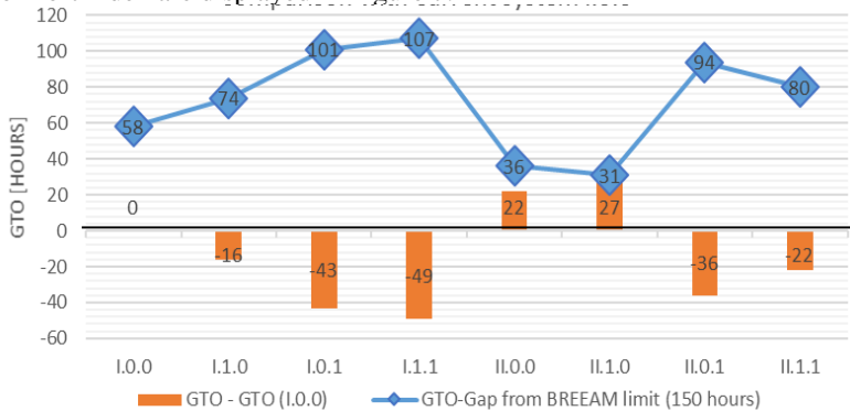
Fig. 7 – GTO index amount for one year simulation compared to simulated current conditions for a single room and to BREEAM temperature comfort requirement.
