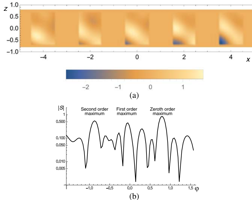
Figure 10. (a) The real part of the contrast current density in the grating. (b) The far field scattering intensity from the grating.
