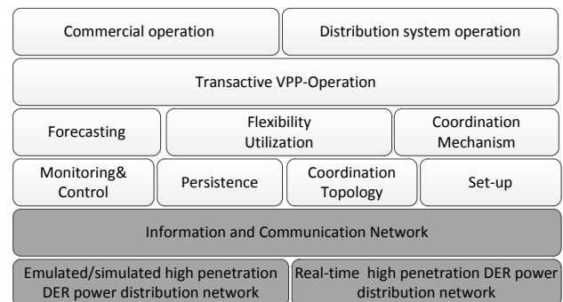
Figure 1 DREAM package structure
