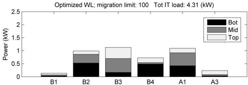
Fig. 9 Optimized IT workload allocation, unlimited migration
