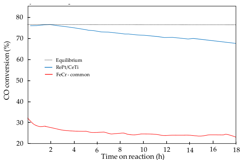
Figure 19. Comparison of CO conversion over the WGS catalyst developed in DEMCAMER and state-of-the-art Fe/Cr catalyst ( 400 \text{ }^\circ\text{C} , SV = 23,230 \text{ L} \cdot \text{h}^{-1} \cdot \text{kg}^{-1} ) [18].
