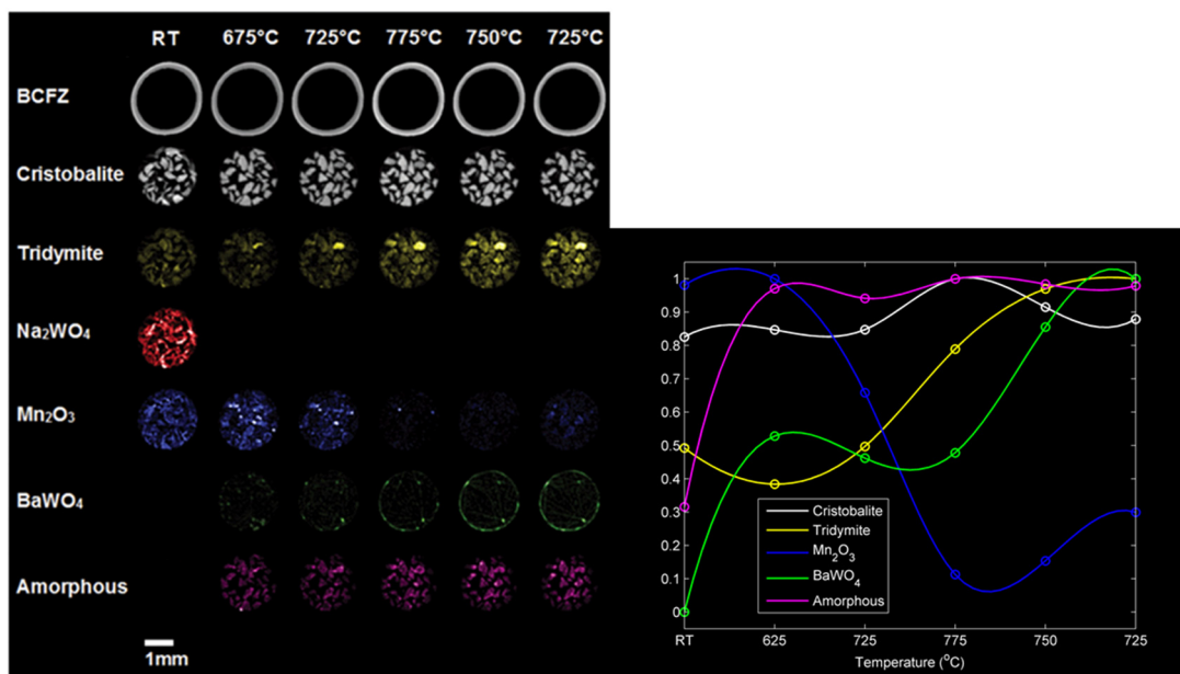
Figure 24. Phase maps obtained from the X-Ray diffraction computed tomography (XRD-CT) data (integrated intensities) of the BaCo x Fe y Zr z O 3-δ BCFZ membrane phase and the catalyst phases: cristobalite and tridymite (SiO 2 polymorphs), Na 2 WO 4 , Mn 2 O 3 , BaWO 4 , and an amorphous phase [28].
