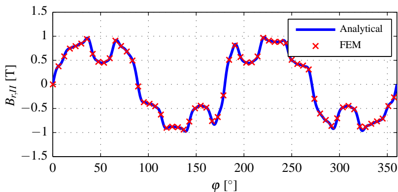
Figure 9. Airgap radial magnetic flux density (region II) of the magnetic gear.
