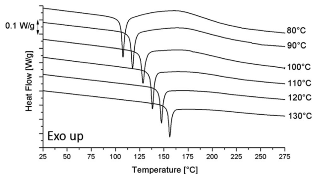
Fig. 5 The DSC heating runs at 10\text{ °C min}^{-1} for the pure epoxy resin after curing at different T_{\text{cure}} and cooling down to -50\text{ °C} at 10\text{ °C min}^{-1} .
