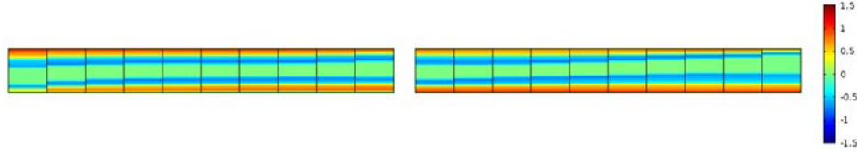
Figure 6: Current distribution normalized to the critical current density in the coil halves situated in the left slot of geometry A, for peak coil currents of 0.45I_c , at t=0.025 seconds.
