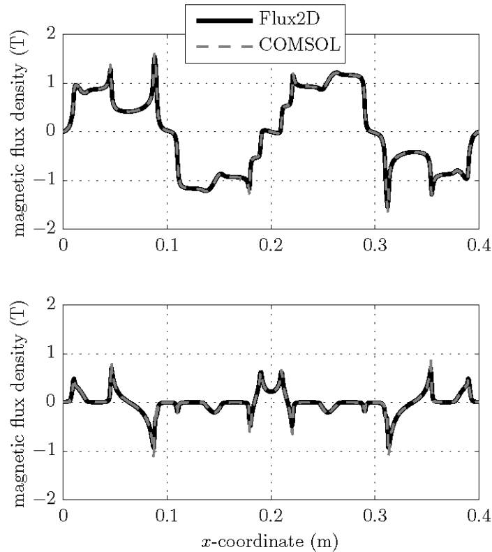
Figure 5: Comparison of calculated air gap magnetic flux density using transient magnetic simulation with H-formulation in COMSOL and static magnetic simulation in Flux2D. Top: x -component of the air gap magnetic flux density. Bottom: y -component of the air gap magnetic flux density.
