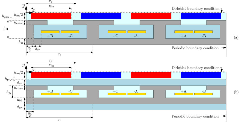
Figure 1: Geometry of one periodic section of the superconducting actuators with moving magnet translator and superconducting stator coils. (a) Geometry A: Cryostat around individual coils, (b) Geometry B: Cryostat around full stator.
