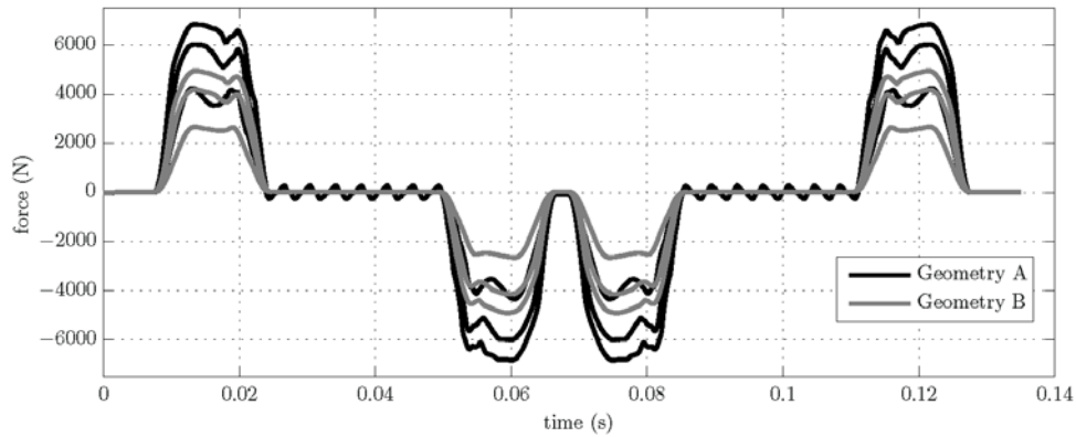
Figure 8 Force as function of time, generated by geometries A and B at peak coil currents of 0.1I_c , 0.2I_c , and 0.3I_c .
