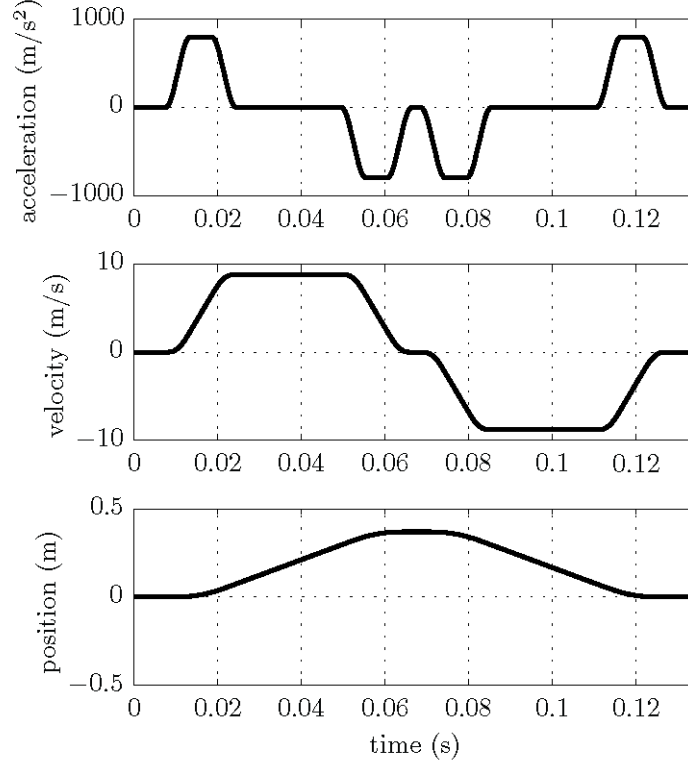
Figure 2: Fourth order motion profile of the translator.
