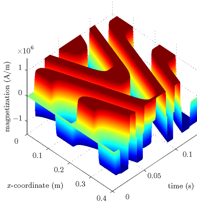
Figure 3: Magnetization of the magnet region, as function of time and x -coordinate.
