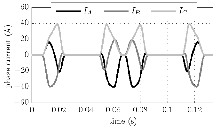
Figure 4: Superconducting coil phase currents.
