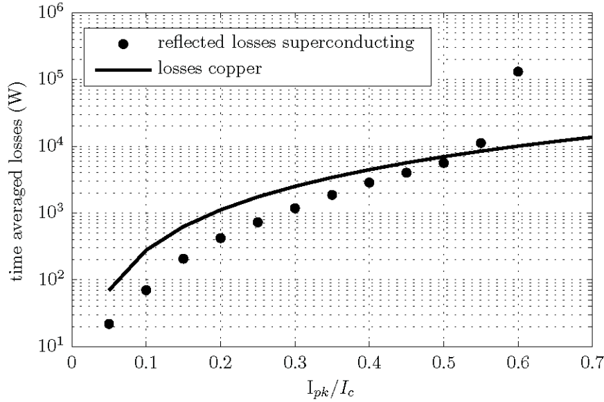
Figure 9: Time averaged reflected losses of the superconducting actuator with geometry A and losses of the copper coil actuator, as function of the ratio of peak current to zero-field critical current.
