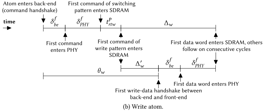
Figure 3.5: Latency experienced by a read or write atom arriving at an idle back-end at the start of a busy period.
