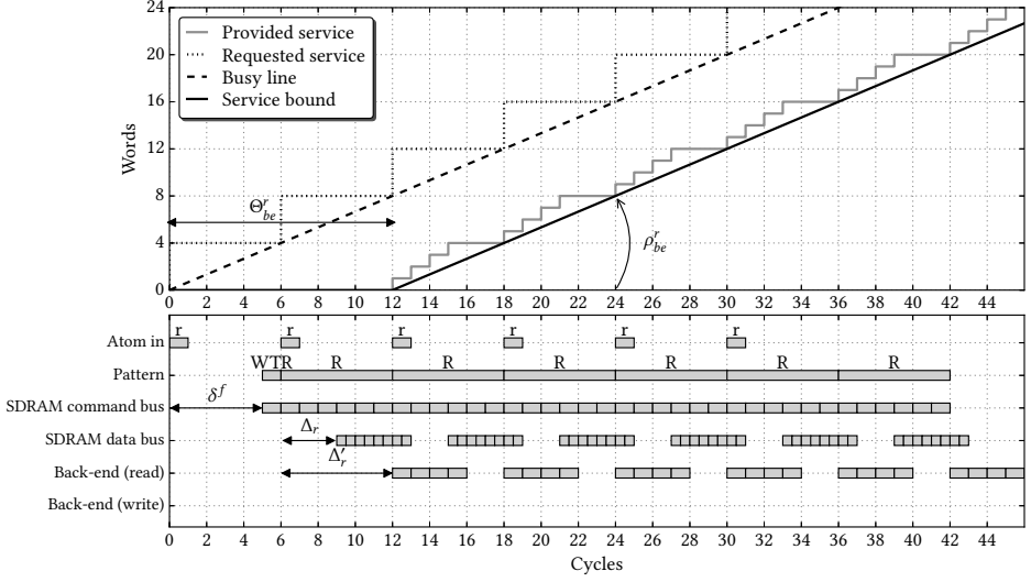
Figure 3.6: Worst-case back-end behavior for continuous reads. In this (fictional) example, we used: t_r^p = 6, t_w^p = 8, t_{rtw}^p = 3, t_{wtr}^p = 1, \Delta_r = 3, \Delta_w = 2, \delta^f = 5, \delta^b = 3 , and each atom is worth 4 words. To simplify the drawing, we assume e_{ref} = 1 .
