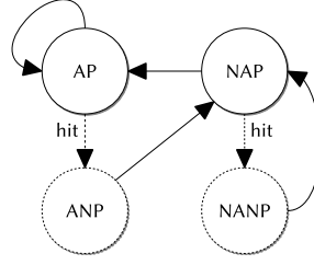
Figure 6.3: Allowed mode transitions. Schedules in dotted modes are not always executed start to finish, but instead begin where the connected mode on their incoming vertex left off when the hit was detected.
