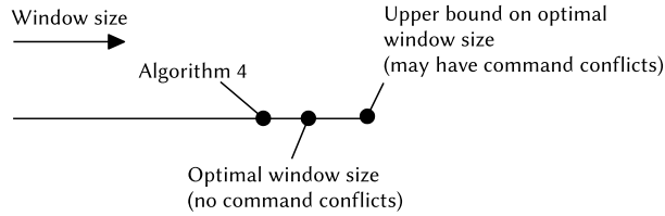
Figure 6.9: We use an upper bound on the optimal window size to determine how far Algorithm 4 can maximally be from the real optimum.
