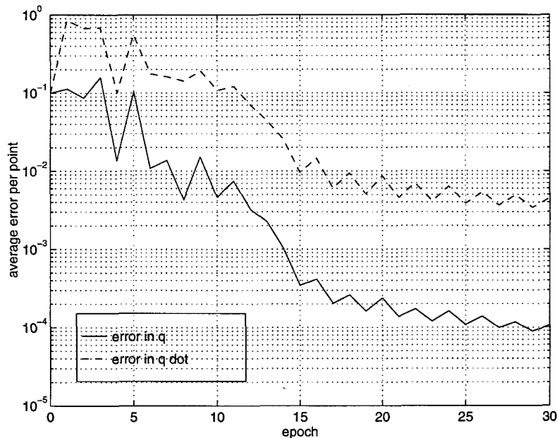
Figure 5: Error per point versus number of epoch for the position ( q ) and the velocity ( q\dot{d} )
