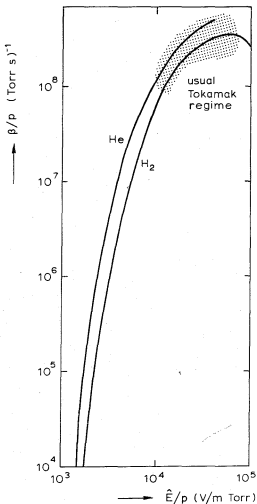
Fig. C.1 \beta/p as a function of reduced electric field strength \hat{E}/p for H_2 and He.
