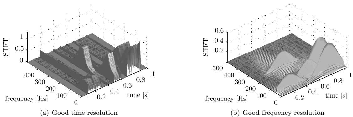
Figure 2.2: STFT for different window lengths
