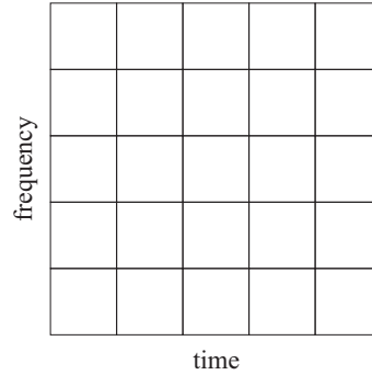
Figure 2.4: Constant resolution time-frequency plane
