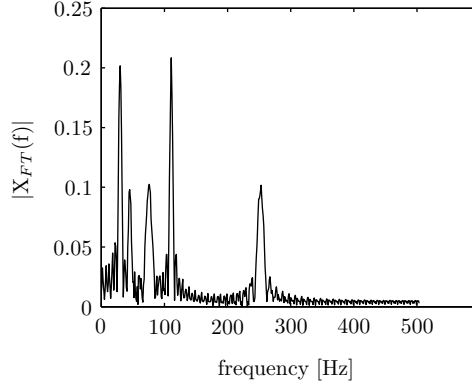
Figure 2.1: Fast Fourier transform
