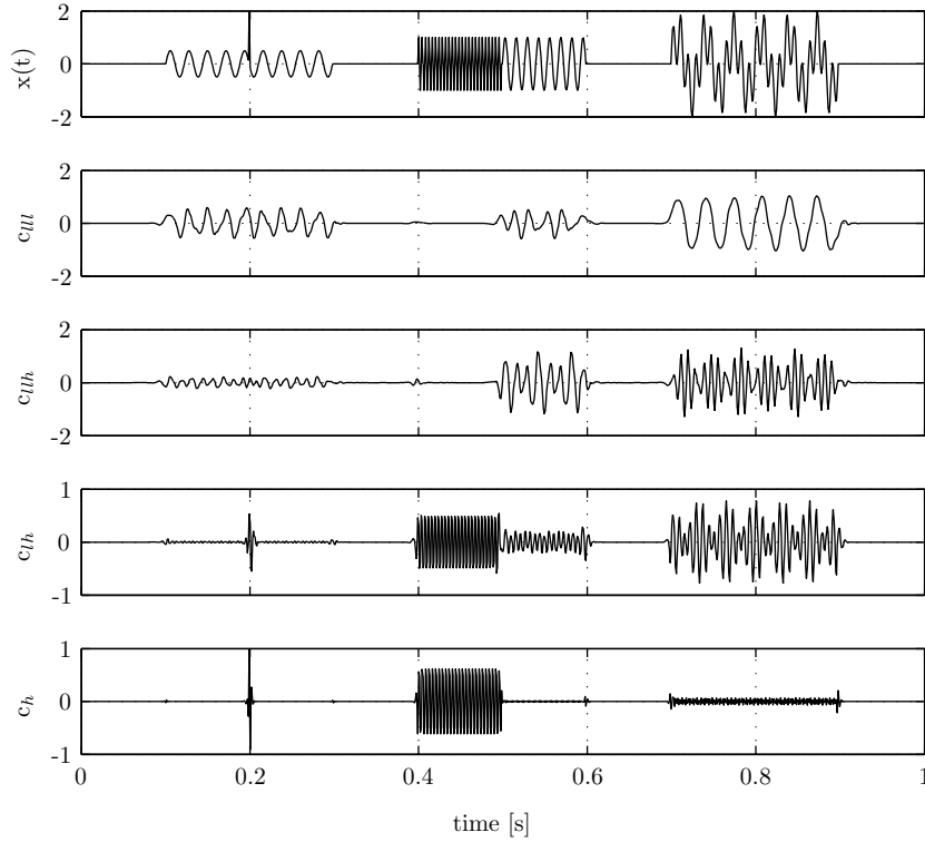
Figure 4.4: Discrete wavelet transform
