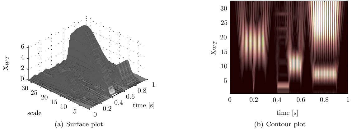
Figure 3.3: Continuous wavelet transform
