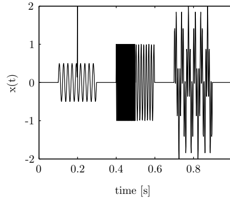
Figure 1.1: Signal x(t)
