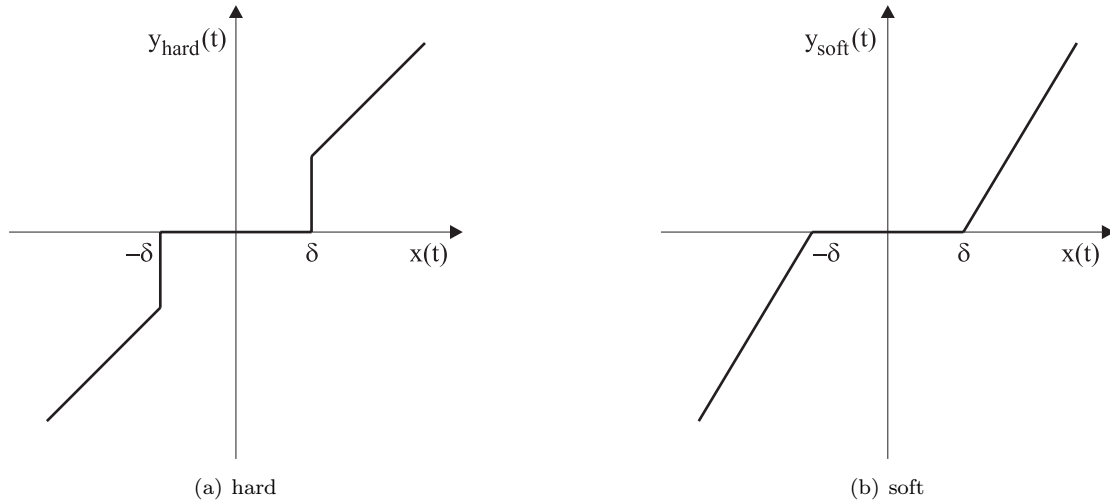
Figure 5.1: thresholding
