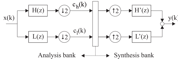
Figure 4.1: Two channel filter bank
