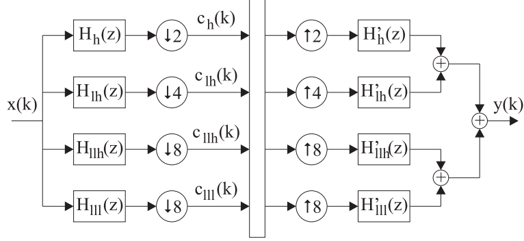
Figure 4.3: equivalent of Fig. 4.2
