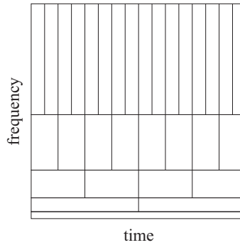
Figure 3.1: Multiresolution time-frequency plane
