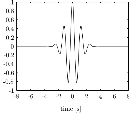
Figure 3.2: Morlet wavelet
