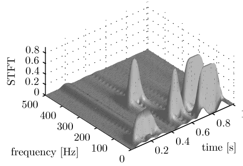
Figure 2.3: STFT with a good compromise between time and frequency resolution
