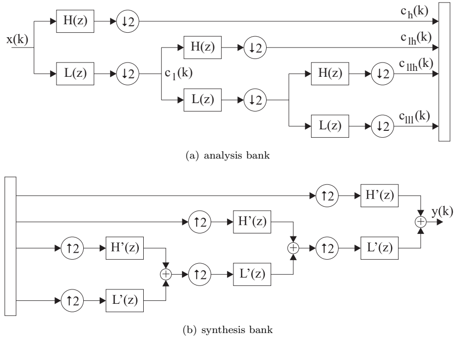
Figure 4.2: three level filter bank
