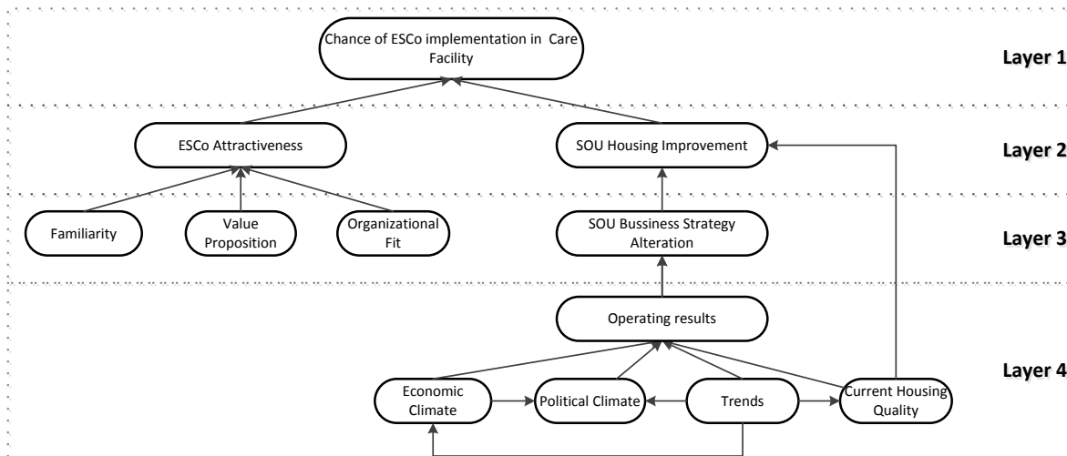
Figure 3: Layer model
