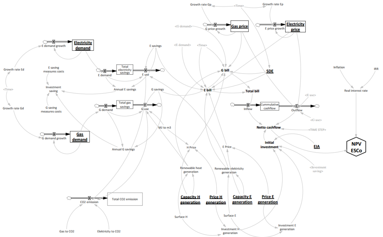
Figure 5 SD model
