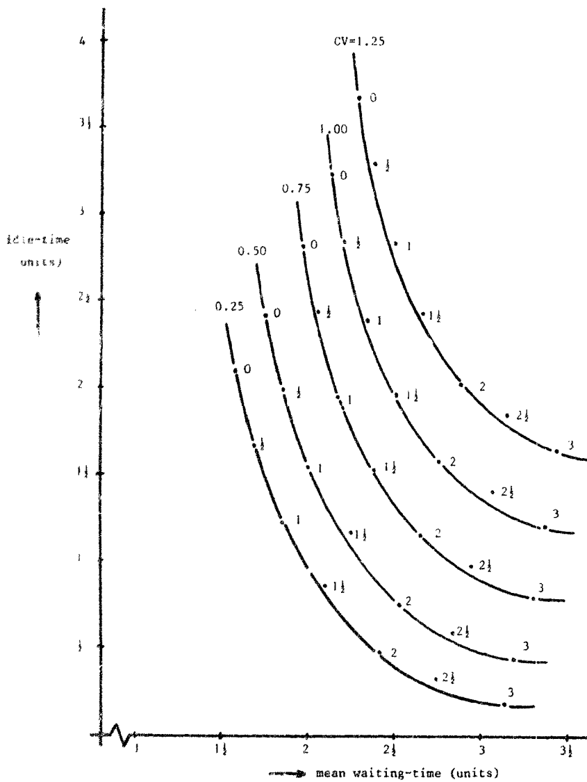
Fig. 1. The waiting and idle-time results for a clinic of 20 patients and different coefficients of variation (average results of 25 sessions). The figures along the curve refer to the system earliness. Waiting-time, idle-time and system earliness are expressed in units, the mean consultation-time taken as one unit of time.
