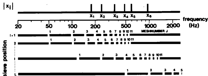
FIG. 7. Example of the harmonic sieve procedure: the component finder produced the set \{177, 242, 360, 485, 600, 960 Hz \} . The components are plotted on a log-frequency scale. The components are then sifted with a harmonics sieve, which has meshes 1 to 11 at harmonic intervals. The mesh width is approximately 8%. The position of the sieve is characterized by, for instance, that of mesh number 1, which starts 50 Hz. Then it moves to 500 Hz in steps of 3%. At each position it is checked which components pass through the sieve. Results for the present example are given in Table I.
