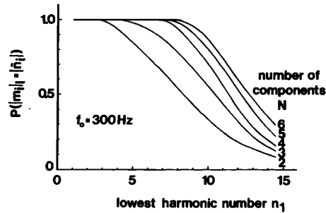
FIG. 3. The probability of correctly estimating the harmonic numbers of the components as a function of the lowest harmonic number presented. Parameter is the number of components. In this example, at f_0 = 300 Hz, it is assumed that all components are successive harmonics (after Goldstein et al. , 1978).
