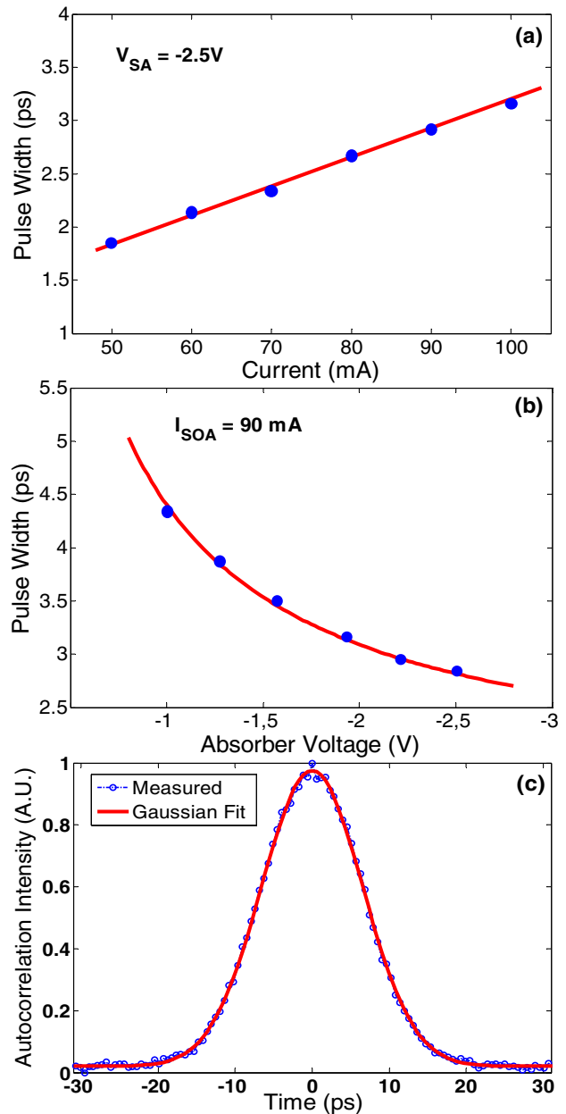
Fig. 7. (a) Pulsewidth versus gain section current level at fixed V_{\text{SA}} ; (b) pulse width versus reverse absorber voltage at fixed I_{\text{SOA}} ; (c) measured optical pulse shape (blue, line marked with circles) fitted to a Gaussian lineshape (red, continuous line).
