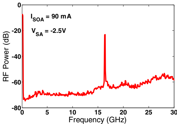
Fig. 6. Electrical spectrum of the OCMLLD; center frequency, 15 GHz; span, 30 GHz; resolution bandwidth (RBW), 1 MHz; video bandwidth (VBW), 1 MHz.
