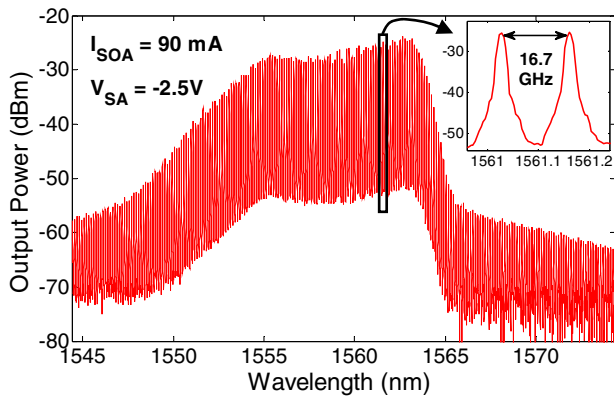
Fig. 5. Optical spectrum of the OCMLLD in the mode-lock state; central wavelength, 1558 nm; span, 30 nm; inset shows the frequency mode spacing; resolution is 0.02 nm.
