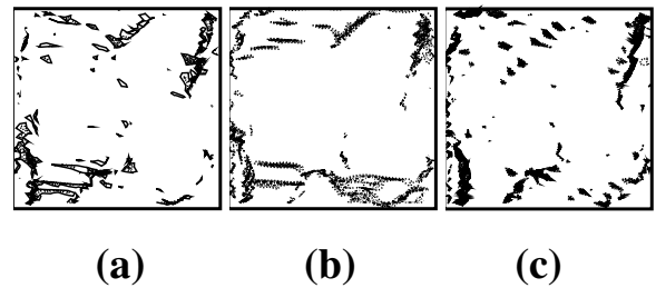
FIG. 3. Contour maps (at t = 400 ) of the spatial locations of (a) the highest local bendings p(\vec{x}, t) < 0.6 , of (b) the highest elastic energies of the beams E_b(\vec{x}, t) , and of (c) the highest contact elastic energies of the spheres E_s(\vec{x}, t) .
