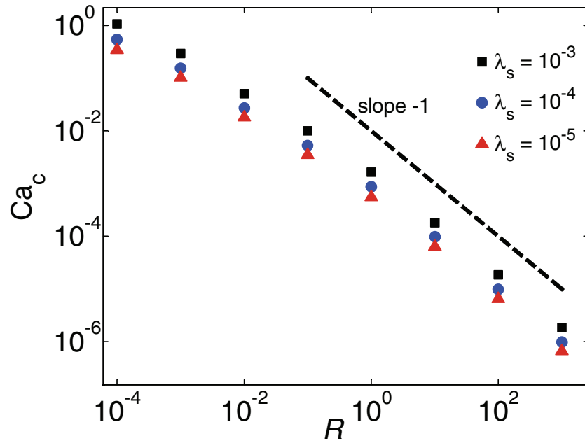
FIG. 9. Critical capillary number Ca_c versus viscosity ratio R for different slip lengths \lambda_s ( \theta_e = 2.8 rad). The dashed line indicates a power law with exponent -1 , which is valid for large R .
