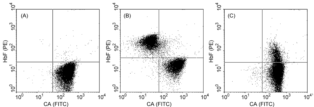
Fig. 1. Dual parameter (CA/HbF) flow cytometric analyses of erythrocytes. Cells are incubated with fluorescently-labeled antibodies against carbonic anhydrase (CA) and HbF. Erythrocytes with fluorescence intensities above the horizontal cut-off lines are designated HbF positive, erythrocytes to the right of the vertical cut-off line are CA positive: (A) normal adult control; (B) artificial sample consisting of adult blood and cord blood; and (C) blood sample of the patient described in this report. For interpretation of the results see text.
