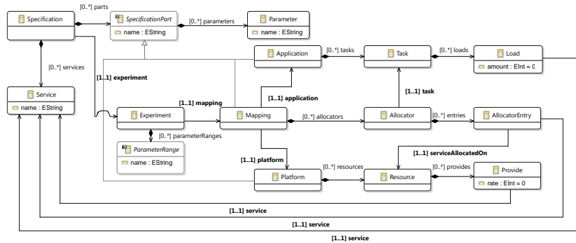
Fig. 4: Simplified excerpt from DseirText metamodel
