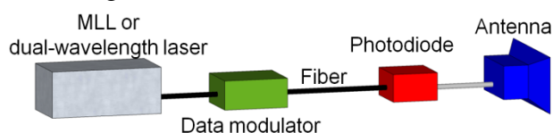
Fig. 1. Block scheme of an optical millimeter wave generator.
