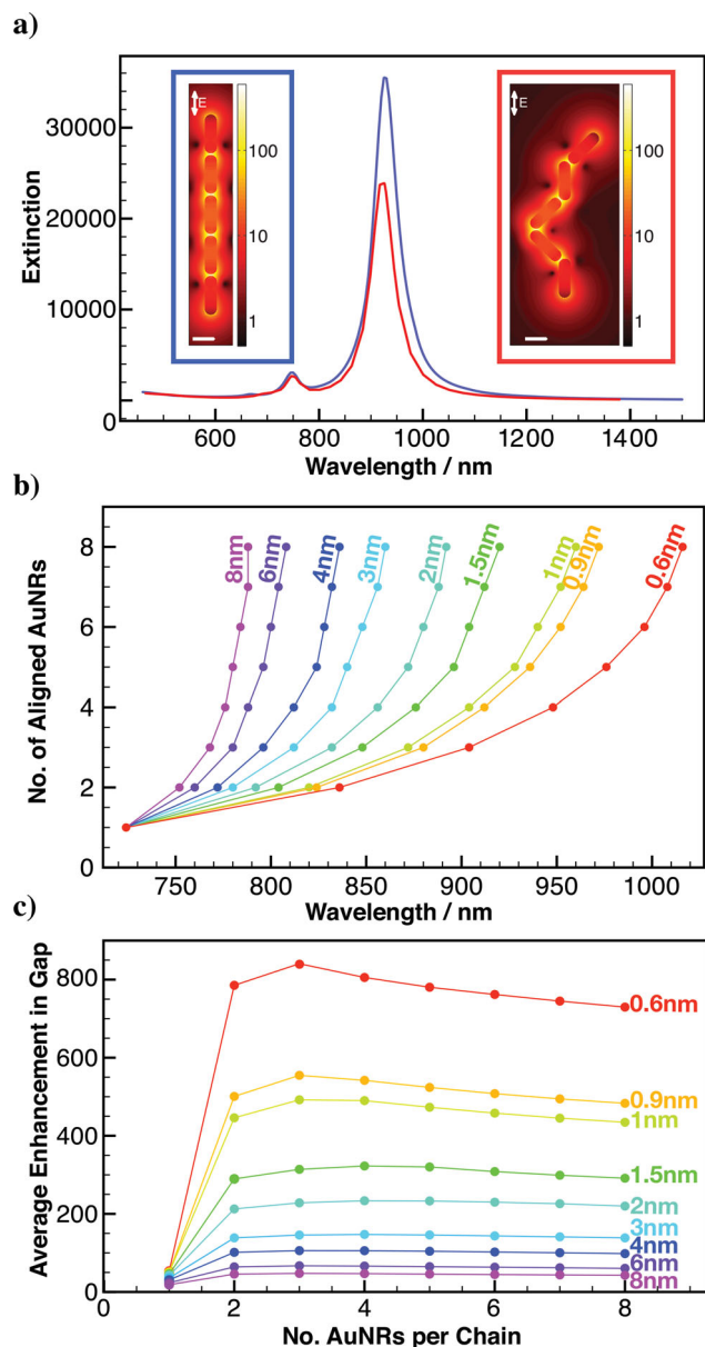
Figure 4. Calculations depicting a) the direct comparison between straight (blue) and “kinked” (red) chains of 36 nm × 11 nm AuNRs at 1 nm separation and field distribution at the lowest energy resonance for each case (insets), b) the effect of increasing chain length, on the extinction spectrum peak for straight chains, with rod separations of 0.6–8 nm and c) the effect of increasing chain length, on the average near field at the center of the gaps, for straight chains with rod separations of 0.6–8 nm.
