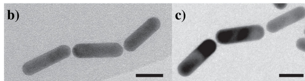
Figure 2. a) Visible to near infrared (Vis-NIR) spectra showing effect of washing untreated AuNRs (blue) against a CB[5] solution (red) twice and peak of the long wavelength resonance \lambda_{\text{max}} vs the number of AuNRs per chain taken from full electrodynamic calculations (green). The inter-rod separation distance is assumed to be of 1 nm in these calculations. b, c) TEM images showing alignment of AuNRs after washing with CB[5]. Scale Bars = 20 nm.
