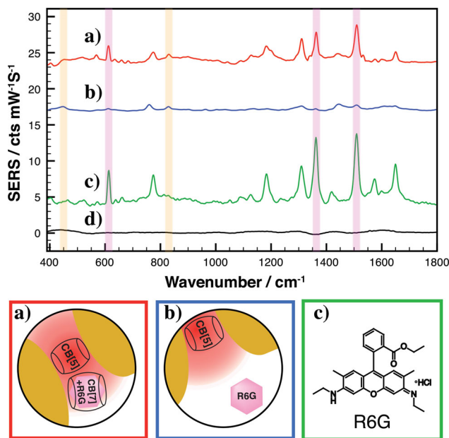
Figure 5. a) SERS spectrum and schematic representation of AuNRs washed against CB[5] and CB[7] in the presence of 100 nM R6G, b) SERS spectrum and schematic representation of AuNRs washed against only CB[5] in the presence of 100 nM R6G, c) Raman spectrum and chemical structure of R6G with characteristic peaks highlighted pink and d) SERS spectrum of AuNRs subjected to the centrifuge wash cycle in the absence of CB[ n ]. Characteristic peaks for CB[ n ] are highlighted orange.
