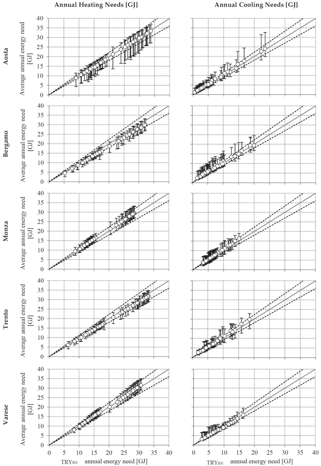
Fig. 2 – Heating and cooling energy needs: the dots are the average energy needs for the considered 10 years, the bars represent the maximum and the minimum in the multi-year series and the dotted lines a deviation of \pm 10\% respect of the TRY EN values
