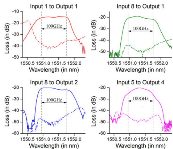
Fig. 6. On-state loss (solid) and off-state loss (dashed). The vertical dashed lines show a bandwidth of 100 GHz. A range of representative paths are presented: Shortest path from input 1 to output 1 (Red), long path from input 8 to output 1 (Green), one of the longest measured paths from input 8 to output 2 (Blue) and worst case passband from input 5 to output 4 (Magenta) are shown.
