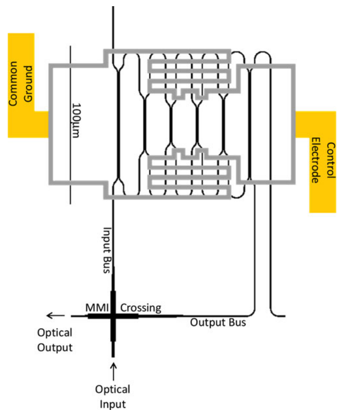
Fig. 2. Mask details for one switch element. The optical waveguides are shown in black. The narrow Ti/Pt micro-heater features are shown in grey, and the wider gold on-chip wiring is shown in orange.
