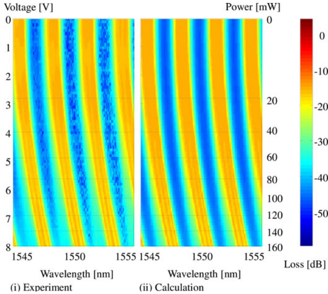
Fig. 4. Thermal tuning of the switch element connecting input 1 to output 1. Experimentally measured optical transfer functions (left) and calculated transfer functions using the transfer matrix model (right).
