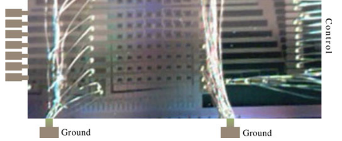
Fig. 3. Photograph of assembled circuit. Wire bonds leading to the left and right of the image are control lines. Wire bonds leading to the bottom edge are the common ground lines.
