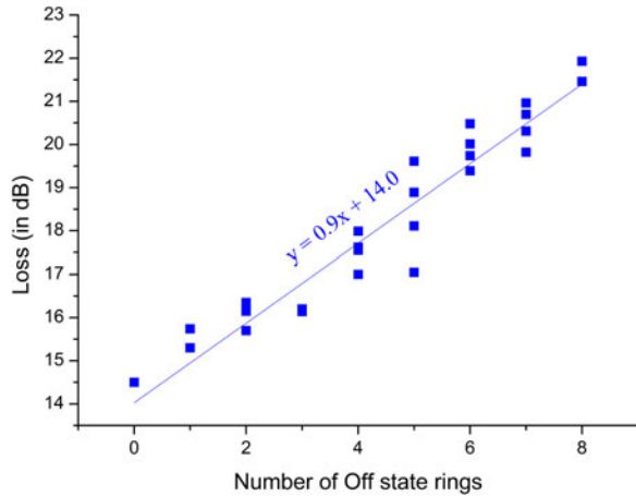
Fig. 7. Fibre coupled losses for paths through the optical switch matrix.
