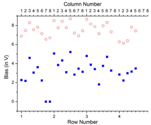
Fig. 5. On state (■) and off-state (○) voltages for an input signal centred at a wavelength of 1551.35 nm for each switch element.
