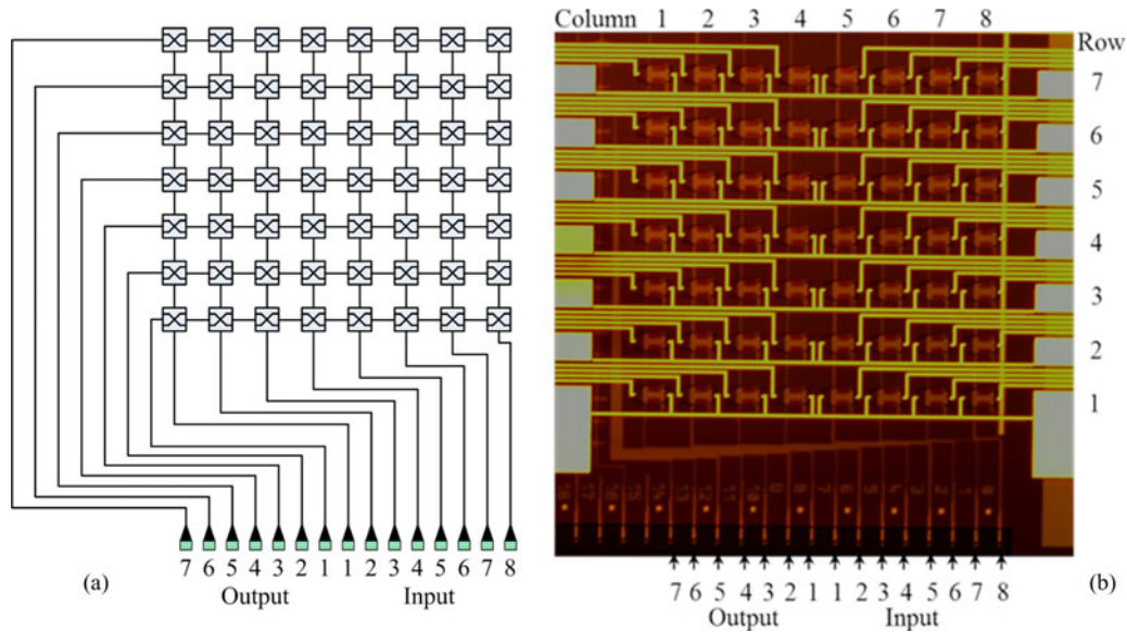
Fig. 1. (a) Schematic layout for the 8 \times 7 matrix switch. (b) Photograph of the full switch matrix with seven rows of eight resonant switches in a crossbar configuration. The inputs and outputs are made via the fiber grating couplers at the bottom of the image.
