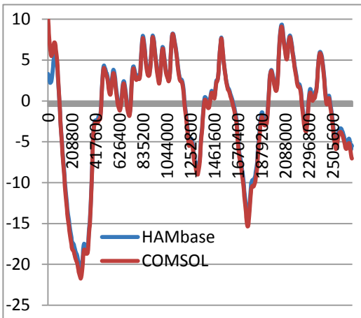
Figure 4 Interior temperatures over time as simulated in HAMBase and COMSOL, climate, façade and volume
