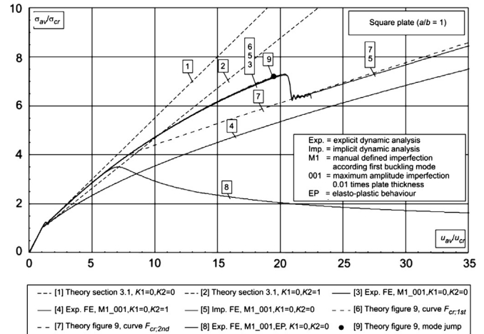
Fig. 12. Results for FE simulations of a square plate.
