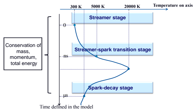
Figure 14. Simulation stages in our physical model and the estimated temperature on the axis of the spark channel in SC N_2 .
