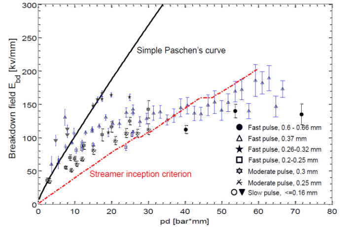
Figure 8. Comparison of the experimental data on the breakdown field E_{bd} in SC N_2 switches with theoretical calculations. Solid line represents Paschen's curve in N_2 ; dashed line represents the calculated breakdown field following the streamer inception criterion with enhanced ionization on the small protrusion at electrode surface.
