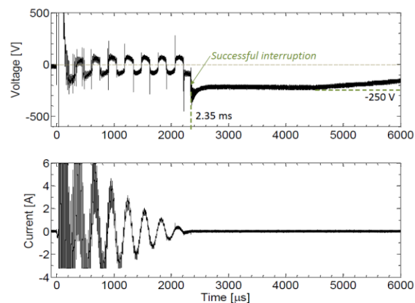
Figure 11. Voltage and current waveforms measured in the SC switch in the arc interruption circuit. Pressure 5 MPa (50 bar), gap width 1.814 mm, L_2 = 9.8 mH, and C_2 = 1 nF. No forced N 2 flushing was supplied during the experiment.
