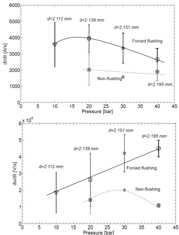
Figure 12. The rate-of-rise of current di/dt and rate-of-rise of recovery voltage du/dt at the moment of successful arc interruption in the SC switch, under situation of forced flushing and no flushing situation, at various pressures.
