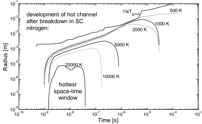
Figure 15. Space-time plot of the N_2 temperature calculated by the model. Radius of spark channel with the region defined as temperature above 1/e \cdot T_{g,t=0} ( T_{g,t=0} : temperature on the axis of the spark channel), 500 K, 1000 K, 2000 K, 5000 K, 10000 K, and 20000 K and respectively.
