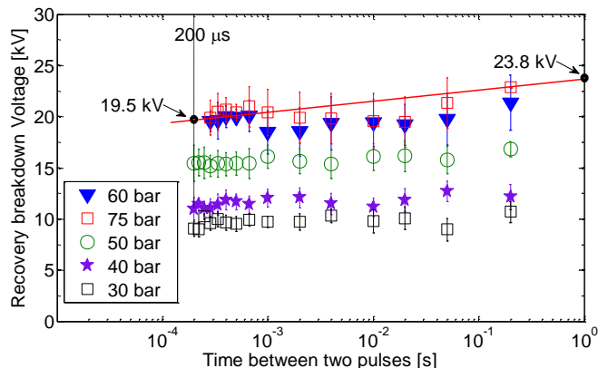
Figure 9. Results from the 1-5000 Hz pulse source: the recovery breakdown voltage of the SC N 2 switch in pre-firing mode as a function of time lag between pulses. The relation with the cold breakdown voltage (= 1 Hz) is estimated by drawing a line from 1 Hz till 5 kHz of the measured data. No SCF flushing is supplied during the experiment.
