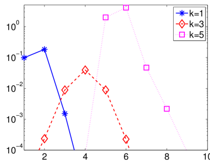
FIG. 2.3. |\eta_j^{(k)}| -factors for j = 1, 2, \dots, 10 for the solutions for which k = 1 (asterisks), k = 3 (diamonds), and k = 5 (squares) for baart of size 100 \times 100 with relative error \nu = 10^{-2} in \mathbf{b} .
