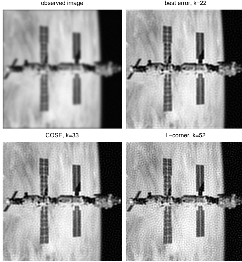
FIG. 5.3. Deblurring of the SPACESTAT test image with \rho_1 = 0.2 , \nu = 10^{-2} : blurred image (top left), minimum 2-norm error (top right), COSE method (bottom left), and L-corner method (bottom right).
