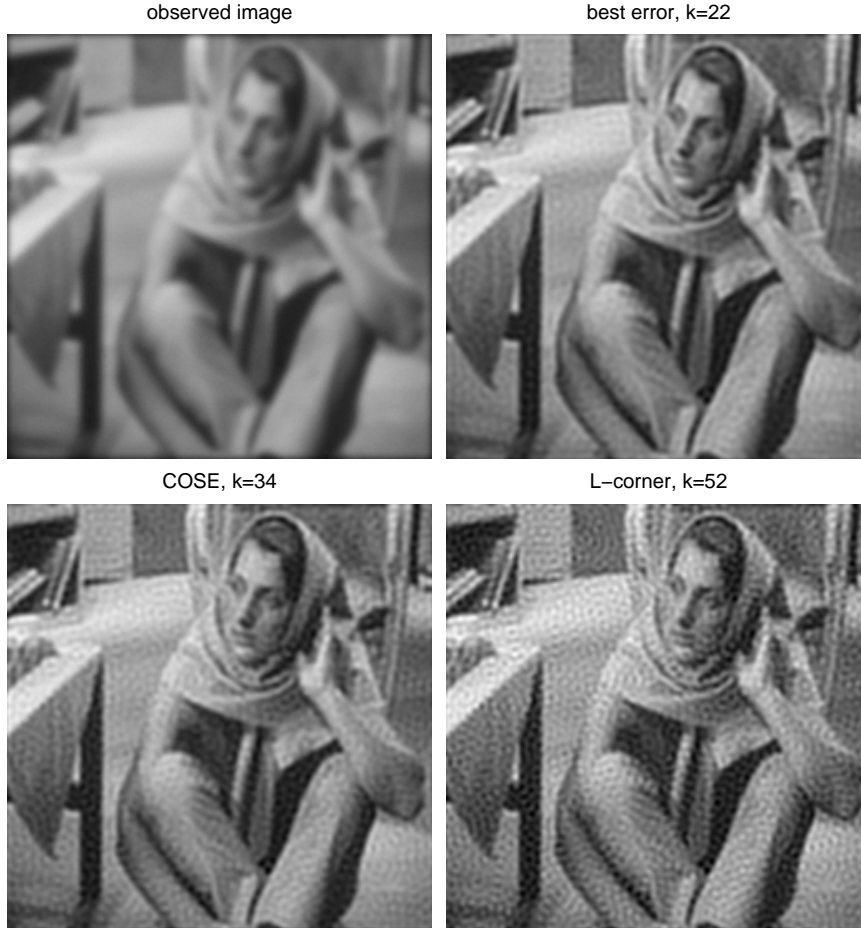
FIG. 5.2. Deblurring of the BARBARA test image with \rho_1 = 0.2 , \nu = 10^{-2} : blurred image (top left), minimum 2-norm error (top right), COSE method (bottom left), and L-corner method (bottom right).
