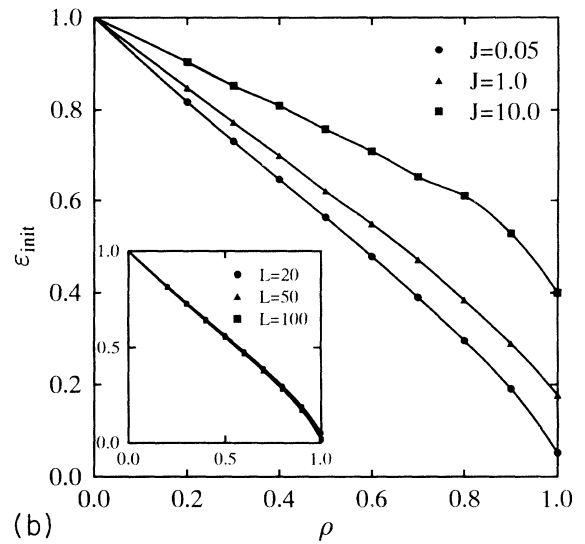
FIG. 7. (a) Breaking stress ( \sigma_{\max} ) and (b) the strain at which the first cell fails ( \varepsilon_{\text{init}} ) as a function of \rho for J=0.05, 1.0 , and 10.0 (bullets, triangles, and squares, respectively) at L=20 . The insets show the result at J=0.05 for system sizes L=20, 50 , and 100 .
