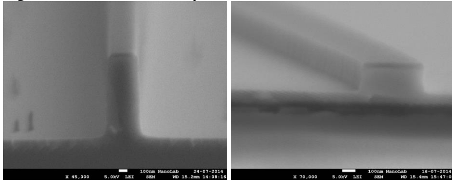
Fig. 1 (a) SEM picture of a 1\ \mu\text{m} deep etched waveguide structure (b) SEM picture of the etched waveguide on InP membrane.
